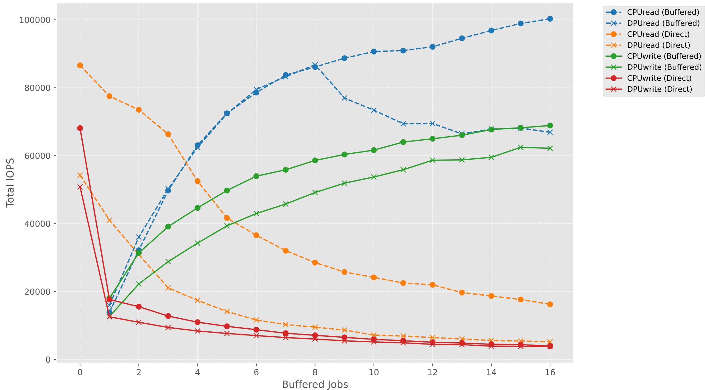
IOPS vs Buffered Jobs (direct1_bufferedN) - SEQ (CPU vs DPU)
